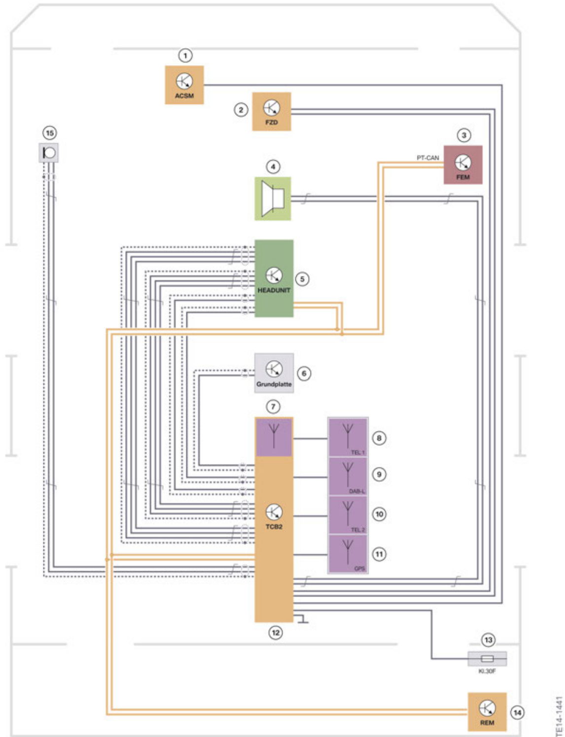
F30 LCI Telematic Communication Box 2 TCB2, roof variant
